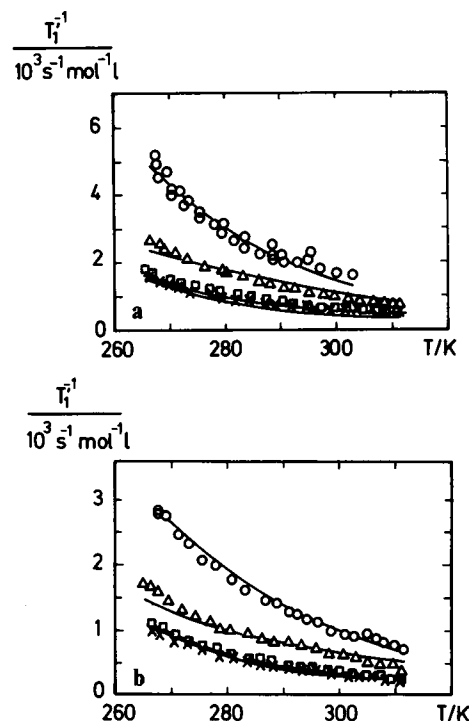
FIGURE 4 Electron-nuclear spin dipole interaction contribution to the water proton relaxation rates of spin-labeled methemoglobin solutions. The specific relaxation rate T'_{\text{in}}{}^{-1} , for four Lamor frequencies are represented by ( \circ ) \nu = 3 \text{ MHz} ; ( \triangle ) \nu = 13 \text{ MHz} ; ( \square ) \nu = 50 \text{ MHz} ; and ( \times ) \nu = 90 \text{ MHz} . The solid lines are calculated using the jump diffusion model, Eq. 5, with parameters given in Table 2. (a) MalSI spin label bound to cys \beta 93 ; (b) IaaSI spin label bound to a surface lysine group.
