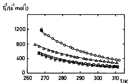
FIGURE 3 Electron-nuclear spin dipole interaction contribution to the water proton relaxation rates, the specific rate T_{1n}^{-1} , of a TEMPO solution in 0.1 M phosphate buffer is shown for four Larmor frequencies. (○) \nu = 3 \text{ MHz} ; (▲) \nu = 13 \text{ MHz} ; (□) \nu = 50 \text{ MHz} ; and (x) \nu = 90 \text{ MHz} . The solid line is calculated using the force-free model for isotropic translational diffusion (Eq. 15) with parameters given in Table 2.
